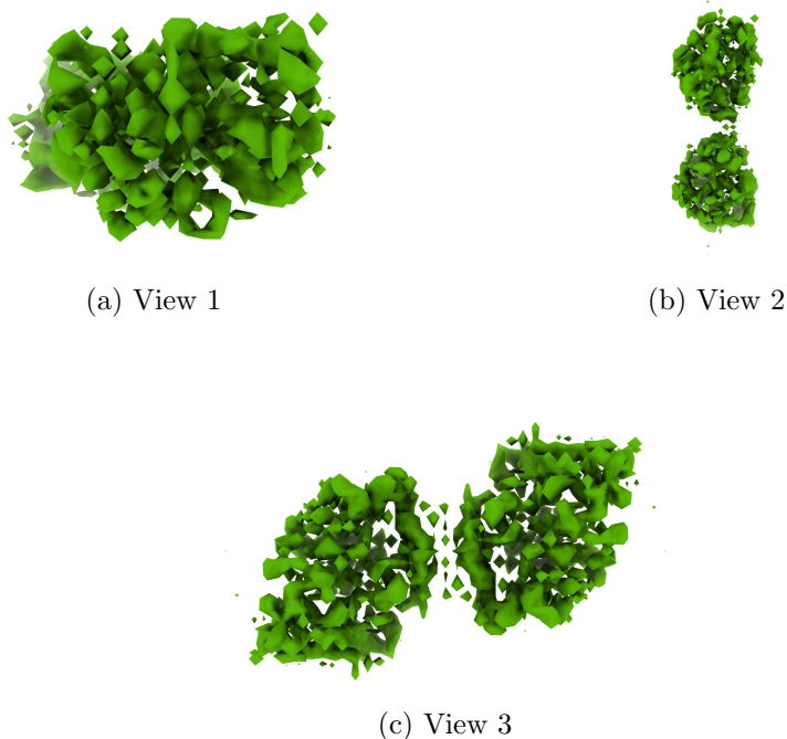
Figure 4: Isosurface at threshold=0.576000. Views generated by ChimeraX at a the following X, Y, Z angles: View 1 (0, -90, -90), View 2 (-90, 0, -90), View 3 (0, 0, 0).
