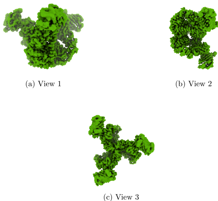
Figure 4: Isosurface at threshold=0.065000. Views generated by ChimeraX at a the following X, Y, Z angles: View 1 (0, -90, -90), View 2 (-90, 0, -90), View 3 (0, 0, 0).
