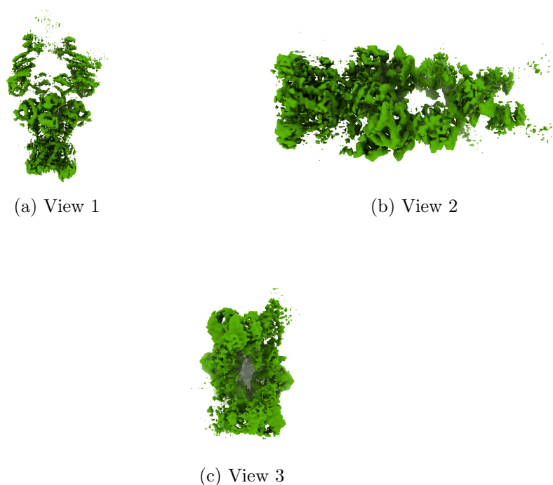
Figure 4: Isosurface at threshold=0.170000. Views generated by ChimeraX at a the following X, Y, Z angles: View 1 (0, -90, -90), View 2 (-90, 0, -90), View 3 (0, 0, 0).
