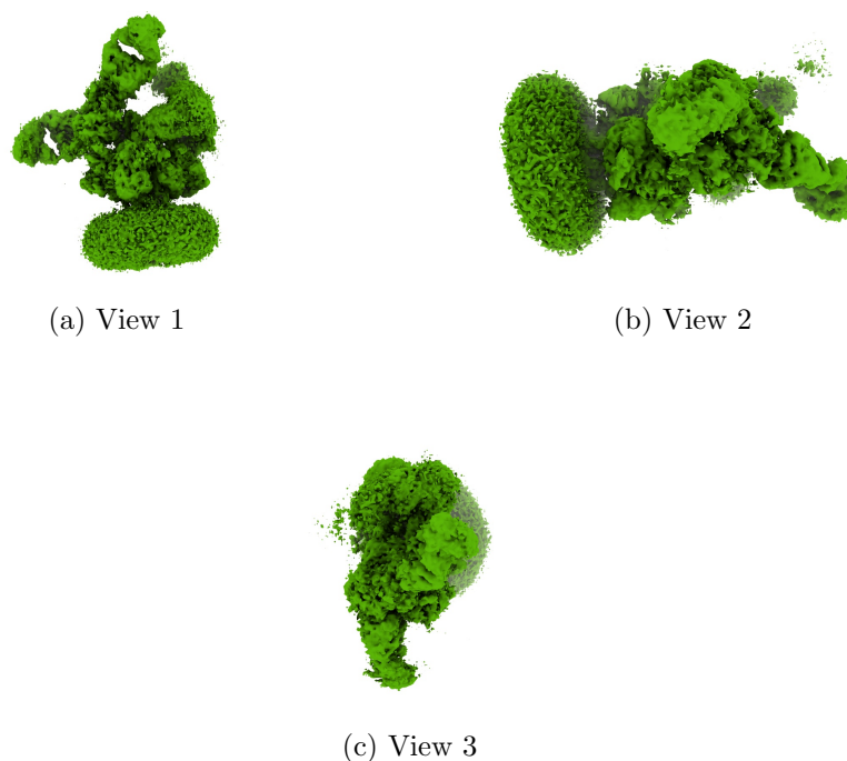
Figure 4: Isosurface at threshold=0.250000. Views generated by ChimeraX at a the following X, Y, Z angles: View 1 (0, -90, -90), View 2 (-90, 0, -90), View 3 (0, 0, 0).
