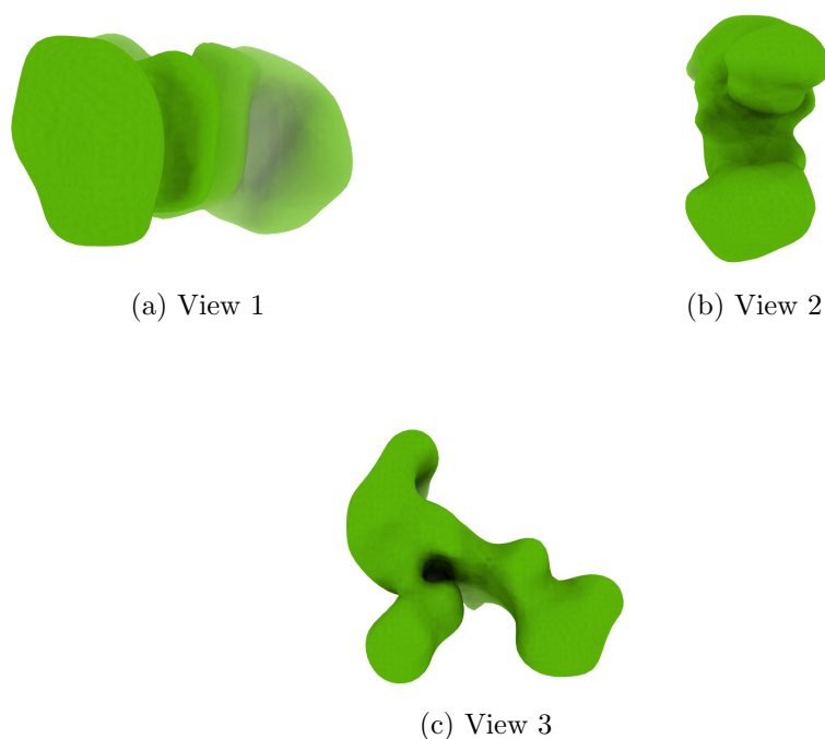
Figure 4: Isosurface at threshold=3.300000. Views generated by ChimeraX at a the following X, Y, Z angles: View 1 (0, -90, -90), View 2 (-90, 0, -90), View 3 (0, 0, 0).
