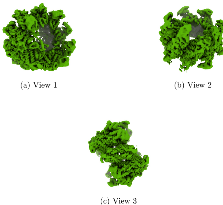
Figure 4: Isosurface at threshold=2.060000. Views generated by ChimeraX at a the following X, Y, Z angles: View 1 (0, -90, -90), View 2 (-90, 0, -90), View 3 (0, 0, 0).
