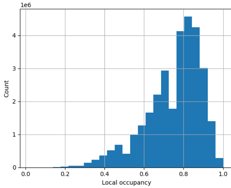
Figure 16: Histogram of the local occupancy according to LocOccupancy.
