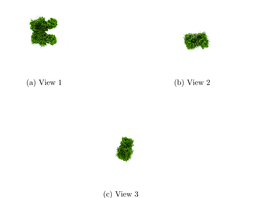
Figure 4: Isosurface at threshold=0.180000. Views generated by ChimeraX at a the following X, Y, Z angles: View 1 (0, -90, -90), View 2 (-90, 0, -90), View 3 (0, 0, 0).
