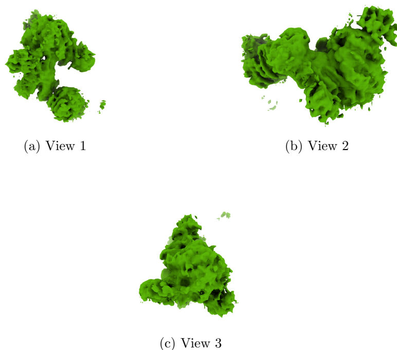
Figure 4: Isosurface at threshold=0.104000. Views generated by ChimeraX at a the following X, Y, Z angles: View 1 (0, -90, -90), View 2 (-90, 0, -90), View 3 (0, 0, 0).
