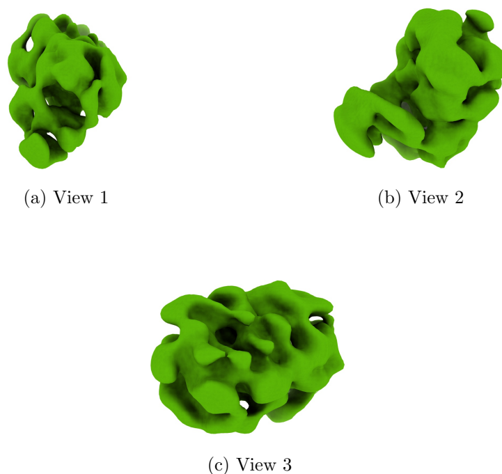
Figure 4: Isosurface at threshold=0.408000. Views generated by ChimeraX at a the following X, Y, Z angles: View 1 (0, -90, -90), View 2 (-90, 0, -90), View 3 (0, 0, 0).
