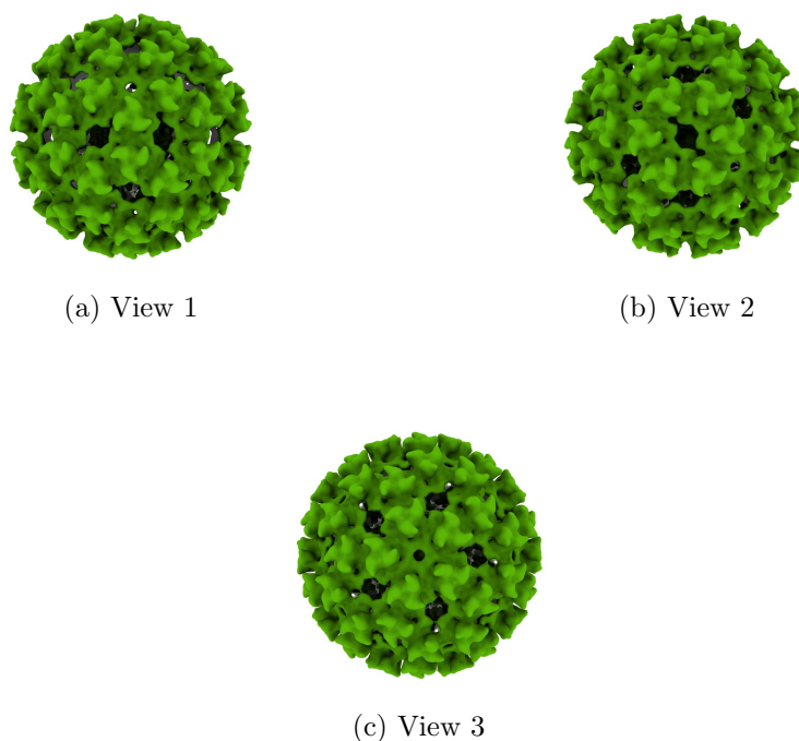
Figure 4: Isosurface at threshold=0.038000. Views generated by ChimeraX at a the following X, Y, Z angles: View 1 (0, -90, -90), View 2 (-90, 0, -90), View 3 (0, 0, 0).
