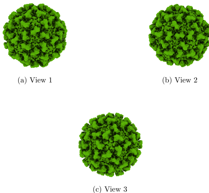
Figure 4: Isosurface at threshold=1.060000. Views generated by ChimeraX at a the following X, Y, Z angles: View 1 (0, -90, -90), View 2 (-90, 0, -90), View 3 (0, 0, 0).
