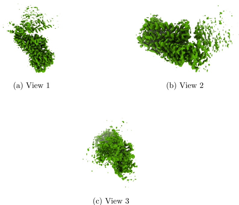
Figure 4: Isosurface at threshold=0.369000. Views generated by ChimeraX at a the following X, Y, Z angles: View 1 (0, -90, -90), View 2 (-90, 0, -90), View 3 (0, 0, 0).
