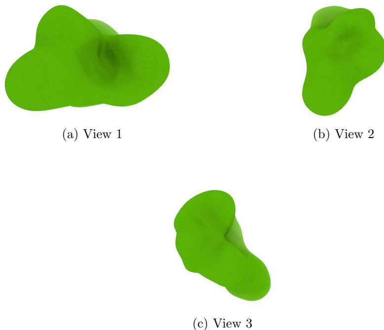
Figure 4: Isosurface at threshold=0.079300. Views generated by ChimeraX at a the following X, Y, Z angles: View 1 (0, -90, -90), View 2 (-90, 0, -90), View 3 (0, 0, 0).
