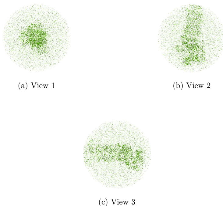
Figure 4: Isosurface at threshold=0.015600. Views generated by ChimeraX at a the following X, Y, Z angles: View 1 (0, -90, -90), View 2 (-90, 0, -90), View 3 (0, 0, 0).
