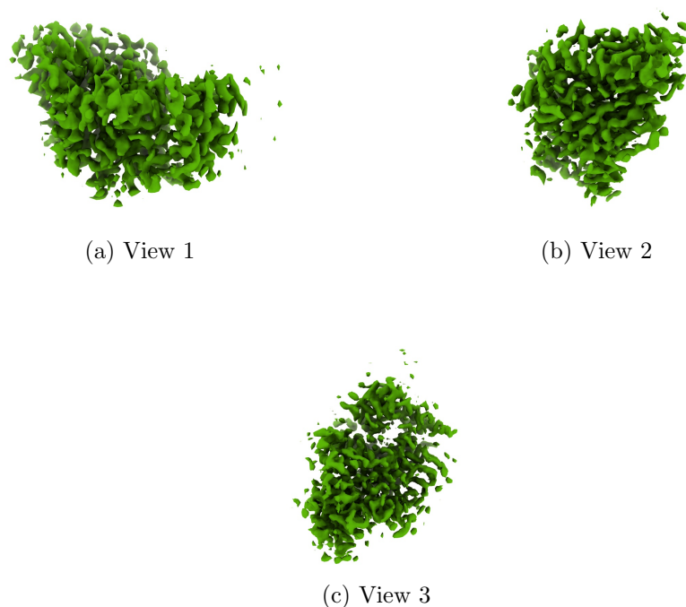
Figure 4: Isosurface at threshold=0.440000. Views generated by ChimeraX at a the following X, Y, Z angles: View 1 (0, -90, -90), View 2 (-90, 0, -90), View 3 (0, 0, 0).
