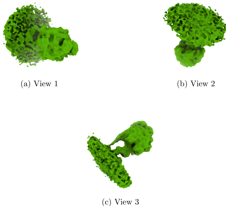
Figure 4: Isosurface at threshold=0.061800. Views generated by ChimeraX at a the following X, Y, Z angles: View 1 (0, -90, -90), View 2 (-90, 0, -90), View 3 (0, 0, 0).
