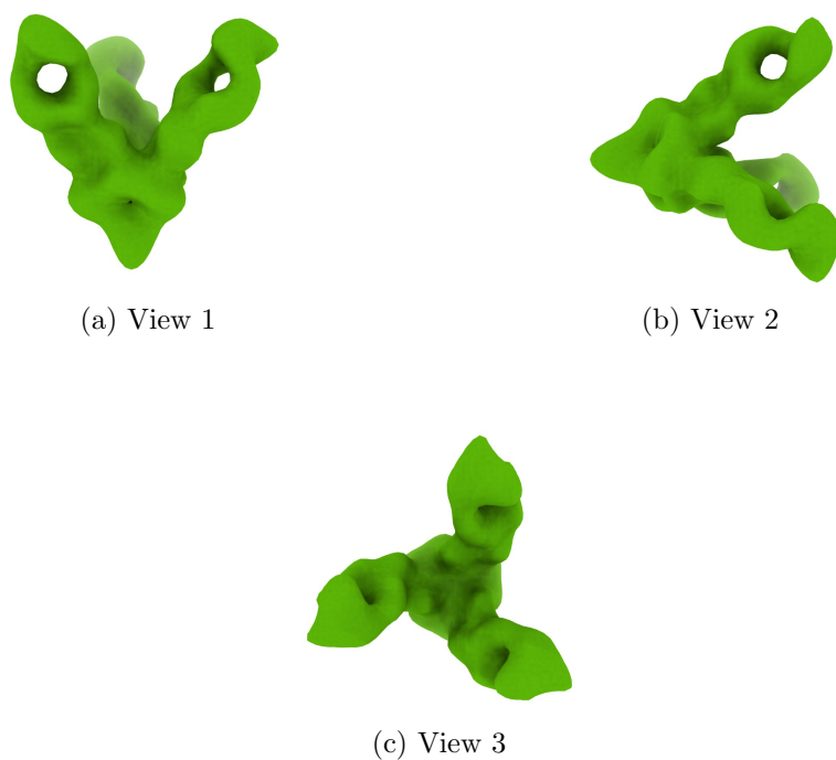
Figure 4: Isosurface at threshold=4.480000. Views generated by ChimeraX at a the following X, Y, Z angles: View 1 (0, -90, -90), View 2 (-90, 0, -90), View 3 (0, 0, 0).
