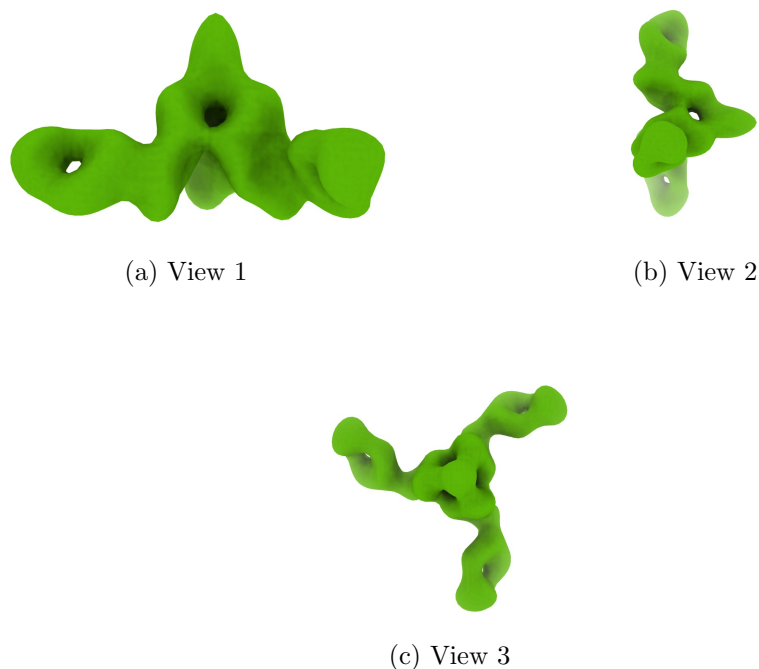
Figure 4: Isosurface at threshold=4.970000. Views generated by ChimeraX at a the following X, Y, Z angles: View 1 (0, -90, -90), View 2 (-90, 0, -90), View 3 (0, 0, 0).
