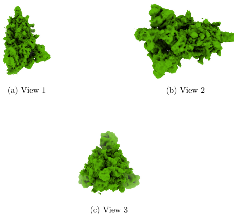
Figure 4: Isosurface at threshold=0.045100. Views generated by ChimeraX at the following X, Y, Z angles: View 1 (0, -90, -90), View 2 (-90, 0, -90), View 3 (0, 0, 0).
