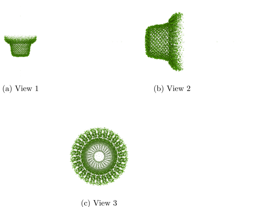
Figure 4: Isosurface at threshold=0.015000. Views generated by ChimeraX at a the following X, Y, Z angles: View 1 (0, -90, -90), View 2 (-90, 0, -90), View 3 (0, 0, 0).
