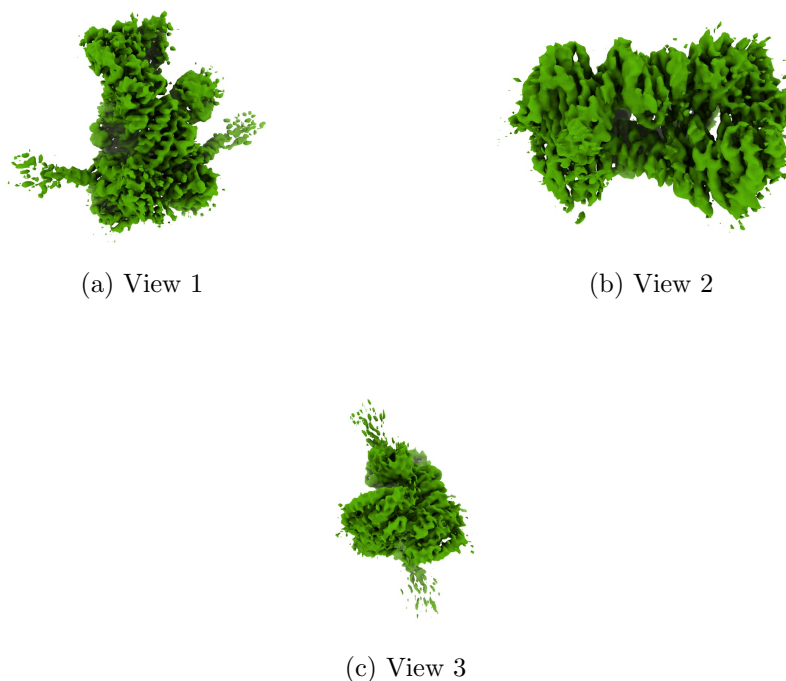
Figure 4: Isosurface at threshold=0.088800. Views generated by ChimeraX at a the following X, Y, Z angles: View 1 (0, -90, -90), View 2 (-90, 0, -90), View 3 (0, 0, 0).
