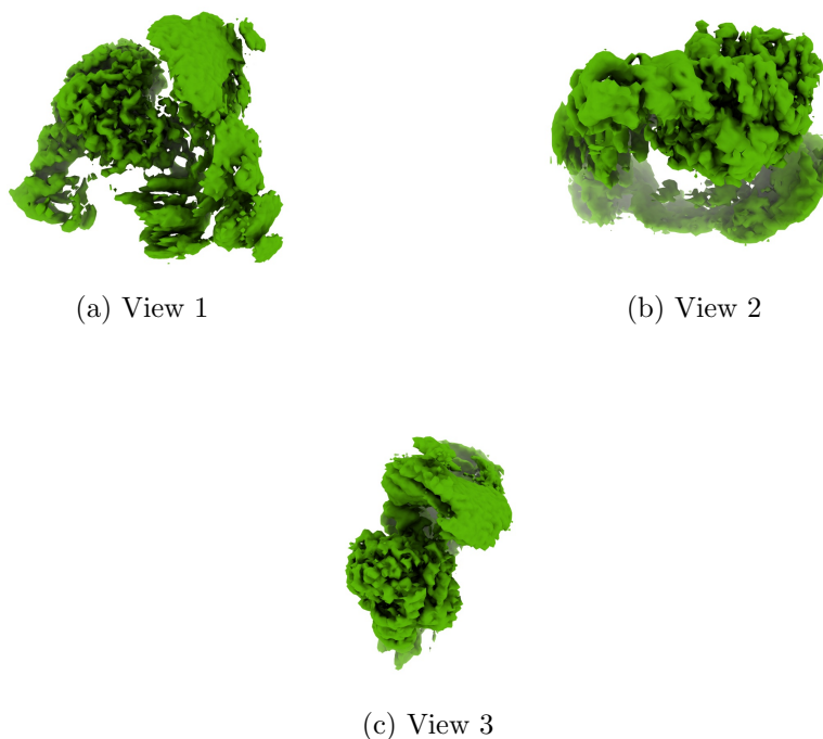
Figure 4: Isosurface at threshold=0.078900. Views generated by ChimeraX at a the following X, Y, Z angles: View 1 (0, -90, -90), View 2 (-90, 0, -90), View 3 (0, 0, 0).
