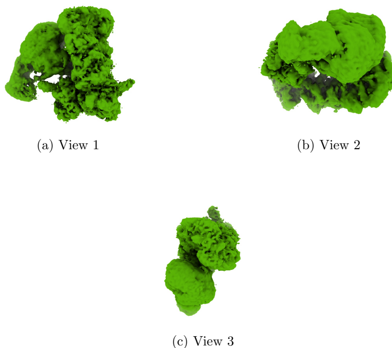
Figure 4: Isosurface at threshold=0.042900. Views generated by ChimeraX at a the following X, Y, Z angles: View 1 (0, -90, -90), View 2 (-90, 0, -90), View 3 (0, 0, 0).
