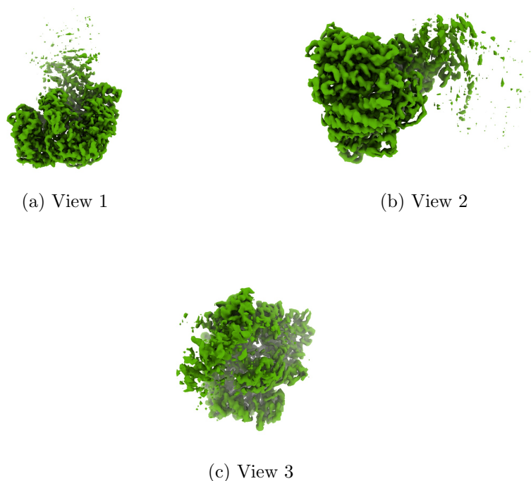
Figure 4: Isosurface at threshold=0.171000. Views generated by ChimeraX at a the following X, Y, Z angles: View 1 (0, -90, -90), View 2 (-90, 0, -90), View 3 (0, 0, 0).
