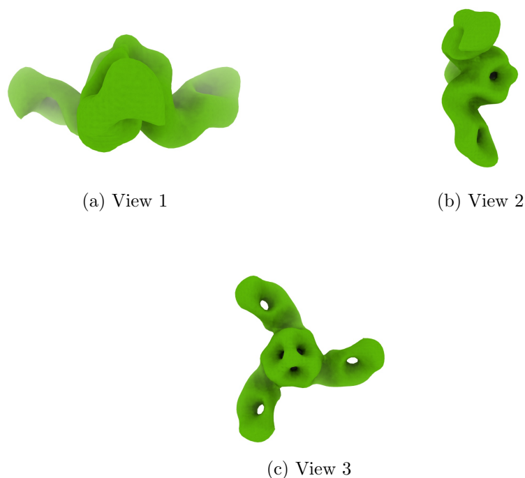
Figure 4: Isosurface at threshold=3.460000. Views generated by ChimeraX at a the following X, Y, Z angles: View 1 (0, -90, -90), View 2 (-90, 0, -90), View 3 (0, 0, 0).
