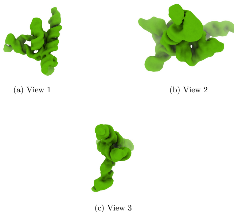
Figure 4: Isosurface at threshold=0.030000. Views generated by ChimeraX at the following X, Y, Z angles: View 1 (0, -90, -90), View 2 (-90, 0, -90), View 3 (0, 0, 0).
