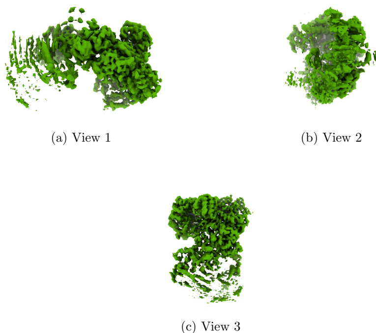
Figure 4: Isosurface at threshold=0.118000. Views generated by ChimeraX at a the following X, Y, Z angles: View 1 (0, -90, -90), View 2 (-90, 0, -90), View 3 (0, 0, 0).
