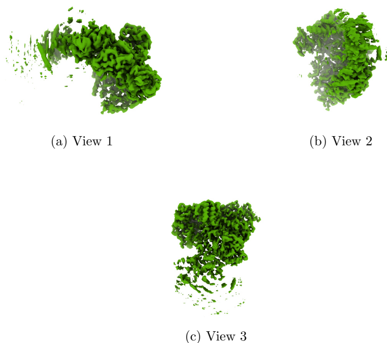
Figure 4: Isosurface at threshold=0.133000. Views generated by ChimeraX at a the following X, Y, Z angles: View 1 (0, -90, -90), View 2 (-90, 0, -90), View 3 (0, 0, 0).
