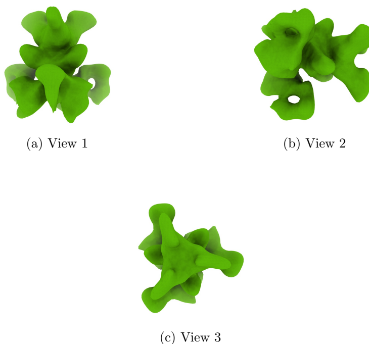
Figure 4: Isosurface at threshold=22.200000. Views generated by ChimeraX at a the following X, Y, Z angles: View 1 (0, -90, -90), View 2 (-90, 0, -90), View 3 (0, 0, 0).
