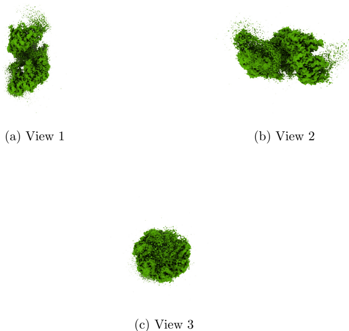
Figure 4: Isosurface at threshold=0.214000. Views generated by ChimeraX at a the following X, Y, Z angles: View 1 (0, -90, -90), View 2 (-90, 0, -90), View 3 (0, 0, 0).
