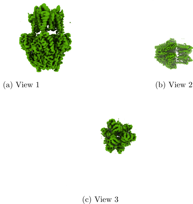
Figure 4: Isosurface at threshold=0.074700. Views generated by ChimeraX at a the following X, Y, Z angles: View 1 (0, -90, -90), View 2 (-90, 0, -90), View 3 (0, 0, 0).
