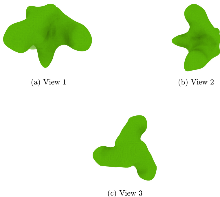
Figure 4: Isosurface at threshold=38.900000. Views generated by ChimeraX at a the following X, Y, Z angles: View 1 (0, -90, -90), View 2 (-90, 0, -90), View 3 (0, 0, 0).
