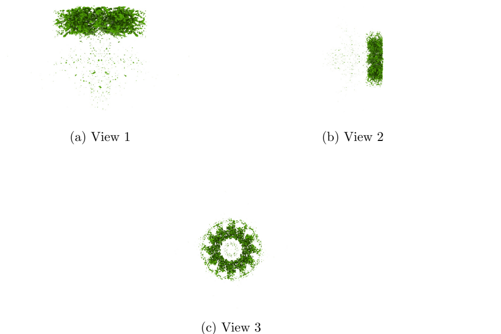
Figure 4: Isosurface at threshold=0.025000. Views generated by ChimeraX at a the following X, Y, Z angles: View 1 (0, -90, -90), View 2 (-90, 0, -90), View 3 (0, 0, 0).
