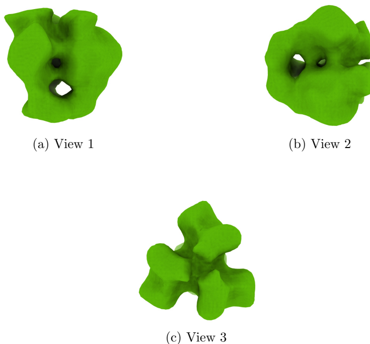
Figure 4: Isosurface at threshold=32.800000. Views generated by ChimeraX at a the following X, Y, Z angles: View 1 (0, -90, -90), View 2 (-90, 0, -90), View 3 (0, 0, 0).
