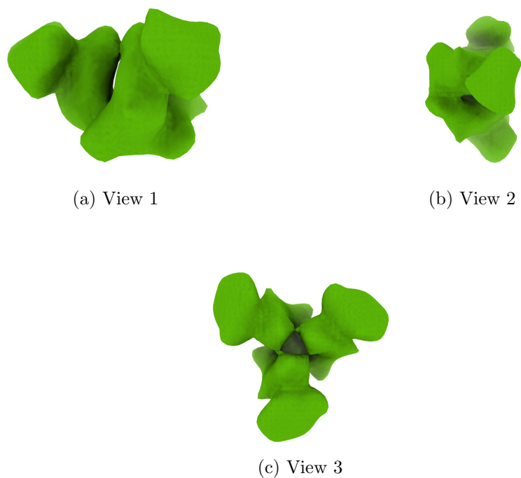
Figure 4: Isosurface at threshold=48.200000. Views generated by ChimeraX at a the following X, Y, Z angles: View 1 (0, -90, -90), View 2 (-90, 0, -90), View 3 (0, 0, 0).
