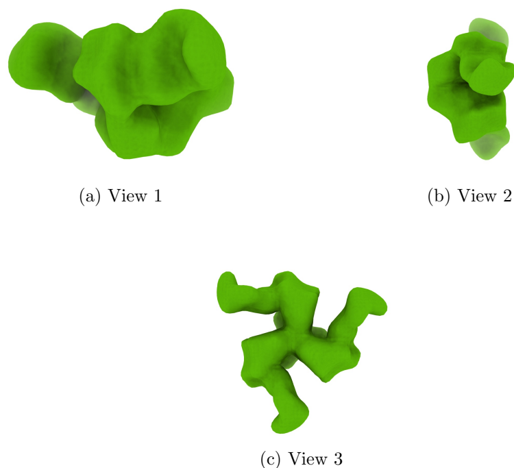
Figure 4: Isosurface at threshold=35.200000. Views generated by ChimeraX at a the following X, Y, Z angles: View 1 (0, -90, -90), View 2 (-90, 0, -90), View 3 (0, 0, 0).
