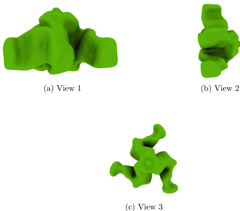
Figure 4: Isosurface at threshold=30.000000. Views generated by ChimeraX at a the following X, Y, Z angles: View 1 (0, -90, -90), View 2 (-90, 0, -90), View 3 (0, 0, 0).
