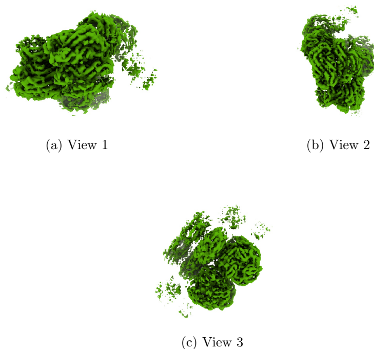
Figure 4: Isosurface at threshold=0.009860. Views generated by ChimeraX at a the following X, Y, Z angles: View 1 (0, -90, -90), View 2 (-90, 0, -90), View 3 (0, 0, 0).
