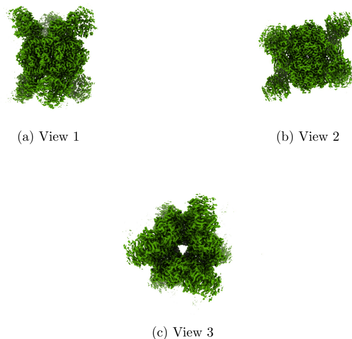
Figure 4: Isosurface at threshold=0.474000. Views generated by ChimeraX at a the following X, Y, Z angles: View 1 (0, -90, -90), View 2 (-90, 0, -90), View 3 (0, 0, 0).
