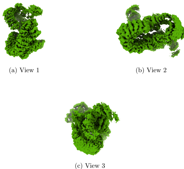
Figure 4: Isosurface at threshold=0.085000. Views generated by ChimeraX at a the following X, Y, Z angles: View 1 (0, -90, -90), View 2 (-90, 0, -90), View 3 (0, 0, 0).
