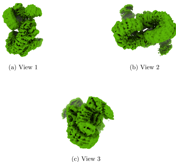
Figure 4: Isosurface at threshold=0.064000. Views generated by ChimeraX at a the following X, Y, Z angles: View 1 (0, -90, -90), View 2 (-90, 0, -90), View 3 (0, 0, 0).
