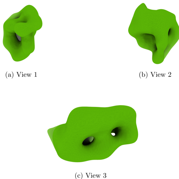
Figure 4: Isosurface at threshold=4.480000. Views generated by ChimeraX at a the following X, Y, Z angles: View 1 (0, -90, -90), View 2 (-90, 0, -90), View 3 (0, 0, 0).
