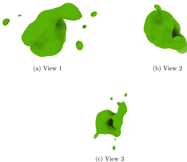
Figure 4: Isosurface at threshold=5.160000. Views generated by ChimeraX at a the following X, Y, Z angles: View 1 (0, -90, -90), View 2 (-90, 0, -90), View 3 (0, 0, 0).
