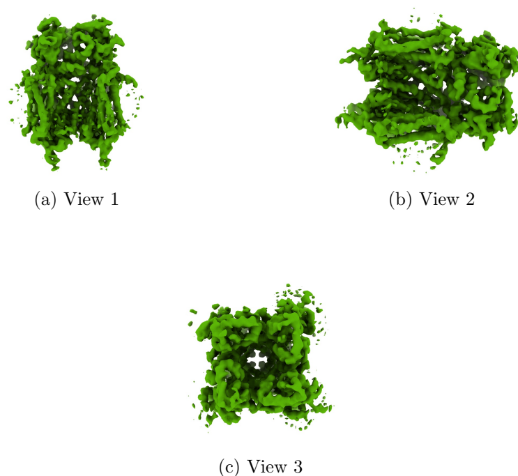
Figure 4: Isosurface at threshold=0.037600. Views generated by ChimeraX at a the following X, Y, Z angles: View 1 (0, -90, -90), View 2 (-90, 0, -90), View 3 (0, 0, 0).
