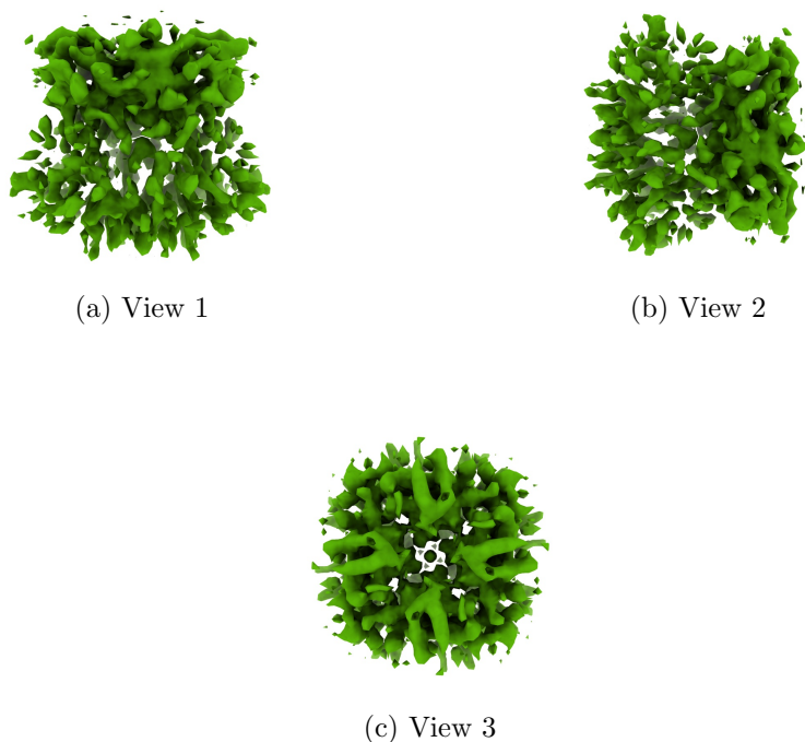
Figure 4: Isosurface at threshold=0.205000. Views generated by ChimeraX at a the following X, Y, Z angles: View 1 (0, -90, -90), View 2 (-90, 0, -90), View 3 (0, 0, 0).
