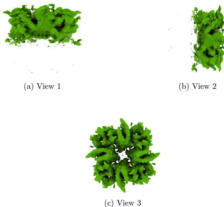
Figure 4: Isosurface at threshold=0.098100. Views generated by ChimeraX at a the following X, Y, Z angles: View 1 (0, -90, -90), View 2 (-90, 0, -90), View 3 (0, 0, 0).
