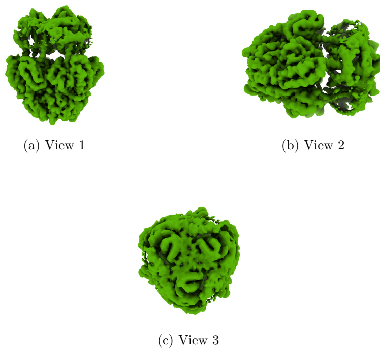
Figure 4: Isosurface at threshold=0.062100. Views generated by ChimeraX at a the following X, Y, Z angles: View 1 (0, -90, -90), View 2 (-90, 0, -90), View 3 (0, 0, 0).
