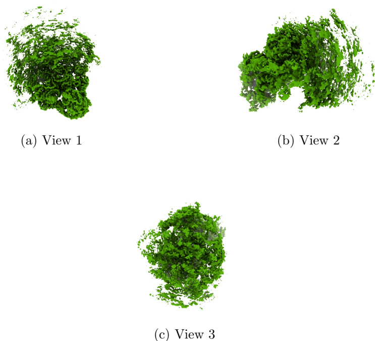
Figure 4: Isosurface at threshold=0.003920. Views generated by ChimeraX at a the following X, Y, Z angles: View 1 (0, -90, -90), View 2 (-90, 0, -90), View 3 (0, 0, 0).
