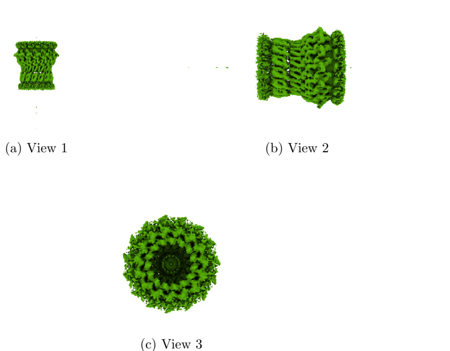
Figure 4: Isosurface at threshold=0.017000. Views generated by ChimeraX at a the following X, Y, Z angles: View 1 (0, -90, -90), View 2 (-90, 0, -90), View 3 (0, 0, 0).
